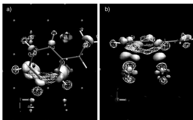
Figure 4. The relaxed styrene molecule on the Ag(100) surface in a 4 \times 4 lateral unit cell, as given by the DFT(LDA) calculations. The induced electron density is shown by the two isosurfaces: electron accumulation (solid grey surface), electron depletion (wireframe). a) Top view: electron depletion at the hydrogen atoms is clearly visible: This leads to an increase in the Löwdin charges (from about +0.13 to around +0.17 ). b) Side view: electron depletion from the aromatic \pi system, as well as from the metal d_{z^2} orbitals, is clearly visible. Electron accumulation in the region between the benzyl ring of the molecule and the surface is characteristic of a weak chemisorption bond.
